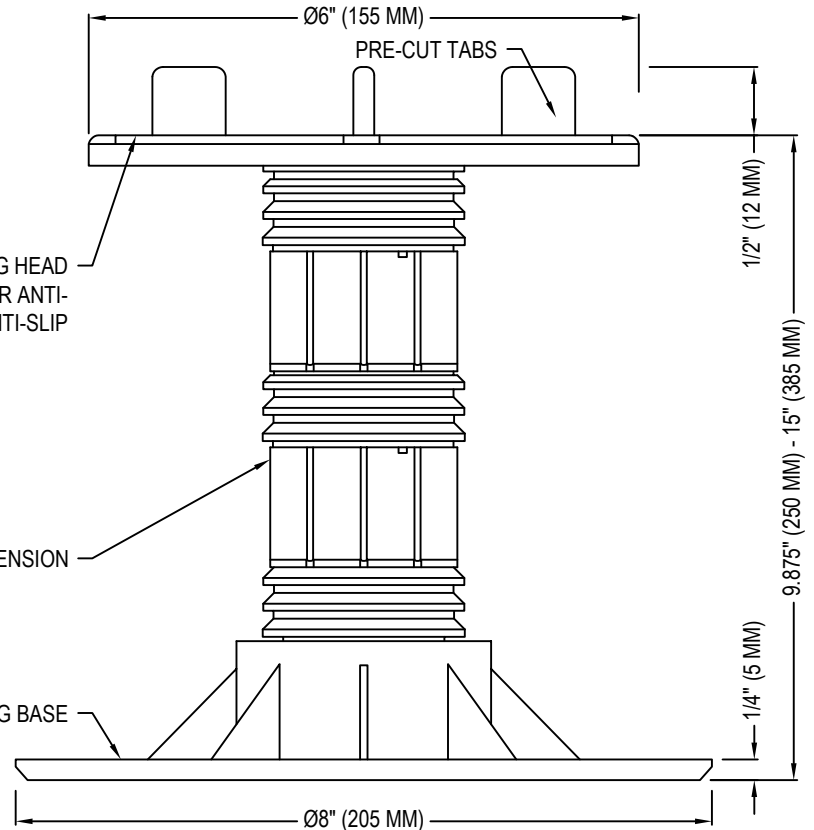
SECTION
